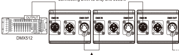
Daisy chaining multiple lights using DMX
