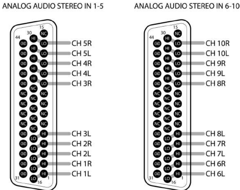
Figure 2.4.4 Analog audio connector pinout
