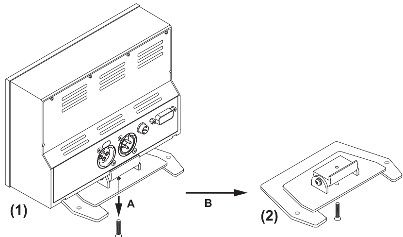
Fig. E 7-1: Removing the table stand
