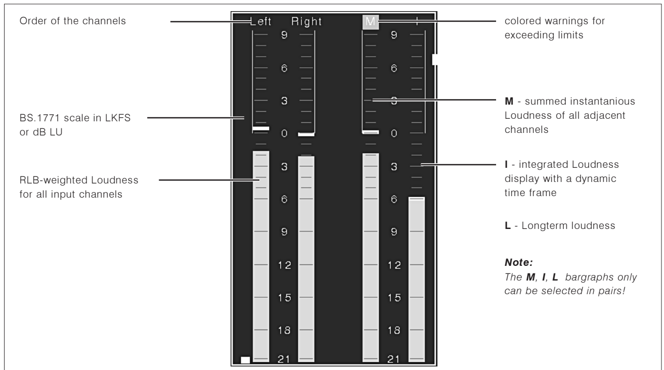
Fig. E 4-4: The Program Meter display in ITU BS.1771 mode (Loudness)
