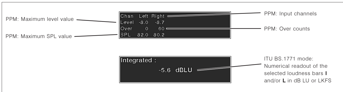
Fig. E 4-20: The Numeric display in Multi Instrument 2 section, above in Program Meter mode PPM, below in Program Meter mode ITU BS.1771
