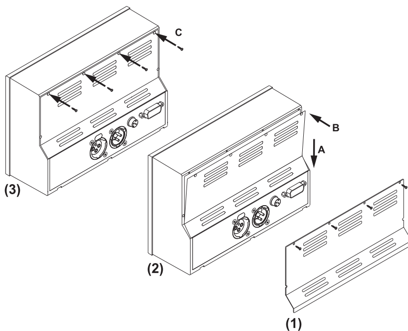
Fig. E 7-12: Mounting the backplane cover
