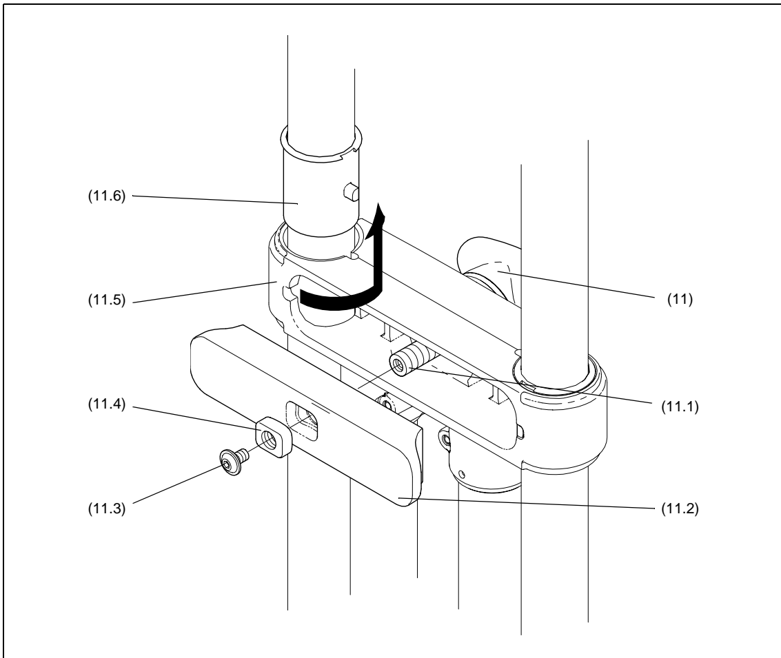
Clamp Sleeves
